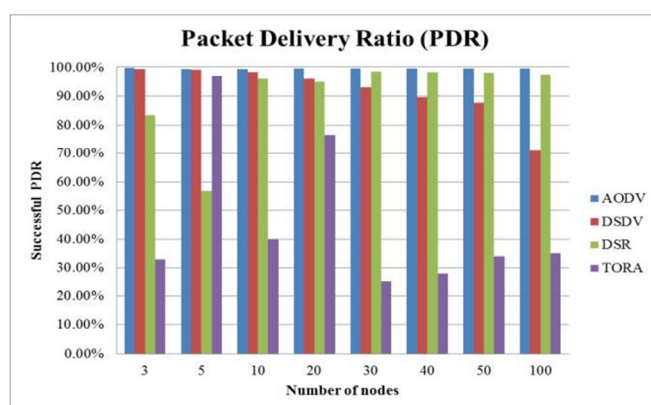
Figure 6.2: Packet delivery ratio(PDR) Analysis IJSEER © 2017 http://www.ijser.org
