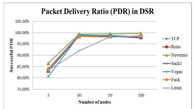
Figure 6.15: PDR analysis in DSR with TCP Agents
